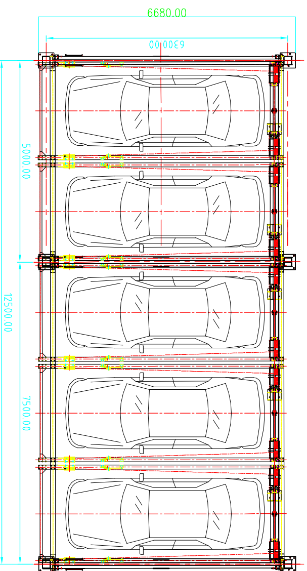
Top view
